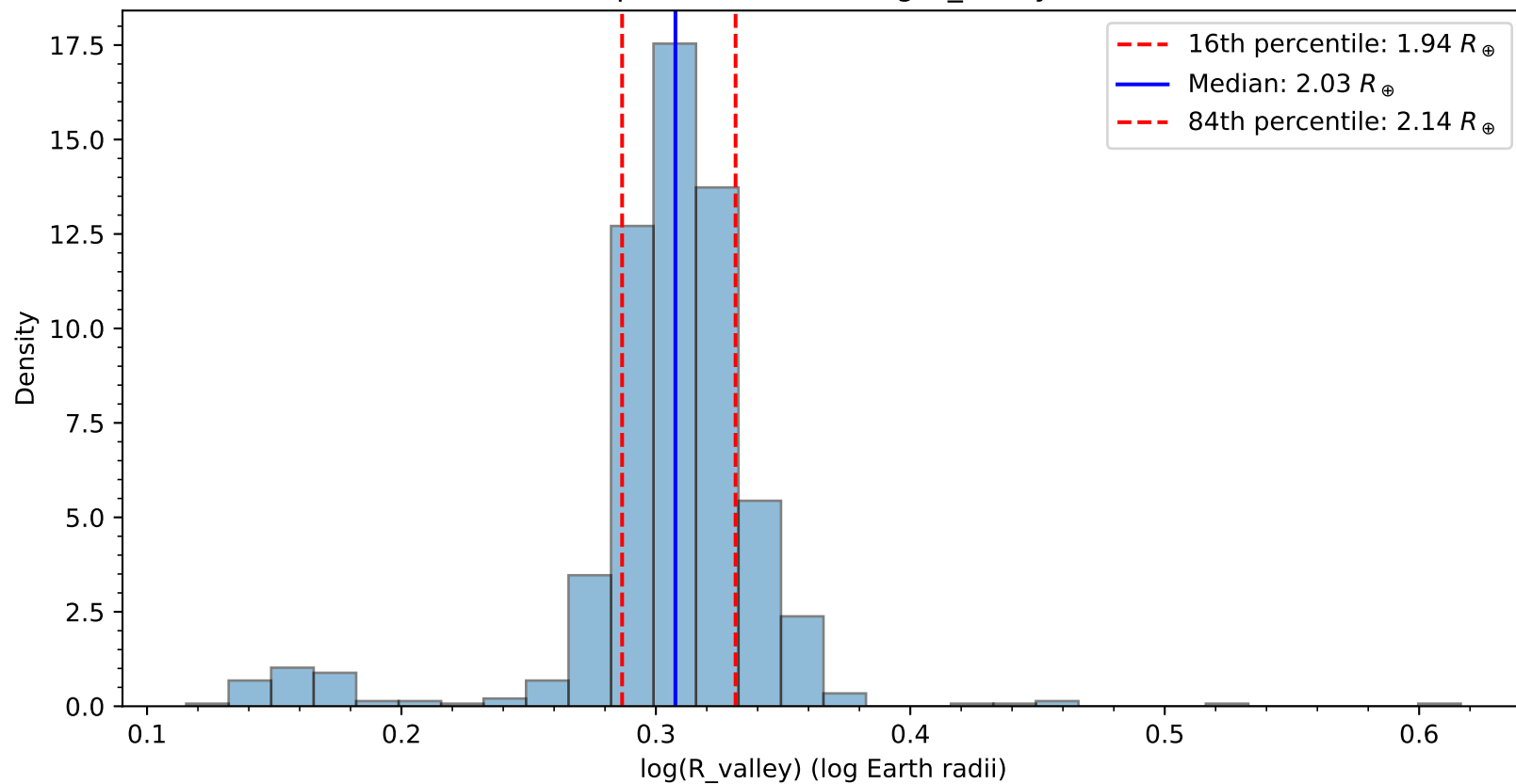
Bootstrap Distribution of \log(R_{\text{valley}}) , bin 3
